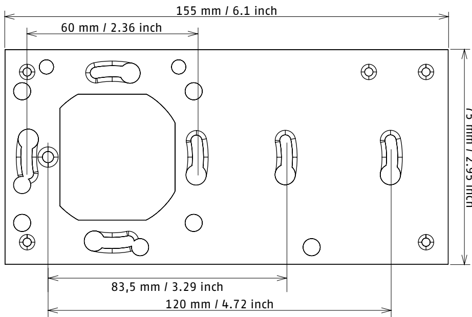
Mouting Plate
