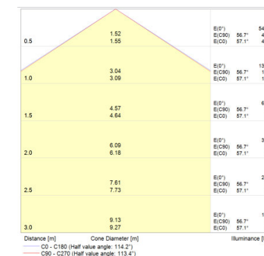
PANEL LED DALI 625 40 W 3000 K
