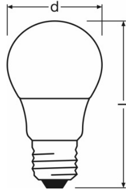
LED STAR CLASSIC A 40 6 W/827 E27 FR, LED STAR CLASSIC A 40 6 W/840 FR E27
