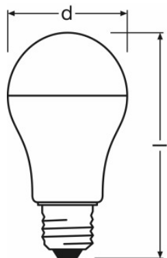
LED STAR CLASSIC A 75 12 W/840 FR E27
